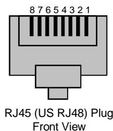
Figure 1-4 RJ45 pin numbering
